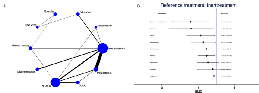
Figure 2 Pain at immediate-term (1 week): network plot (A) and interval plot (B). NSAIDs, non-steroidal anti-inflammatory drugs; SMD, standardised mean difference.
